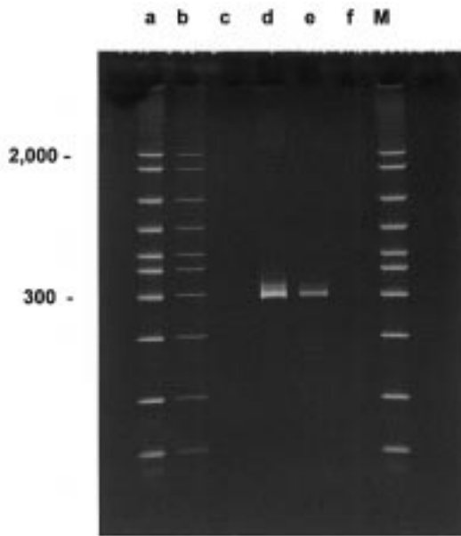
Fig. 4 Destruction of nucleic acid by ESW-L The DNA marker solution was mixed with unelectrolyzed sodium chloride solution (lane b) or ESW-L (lane c) and compared with untreated DNA marker solution (lane a) on the gel. An RNA solution of pAW 109 was mixed with unelectrolyzed sodium chloride solution (lane e) or ESW-L (lane f), and amplified by RT-PCR. The RNA was simply amplified pAW 109 without any treatment (lane d). Lane M indicated marker for bp.
