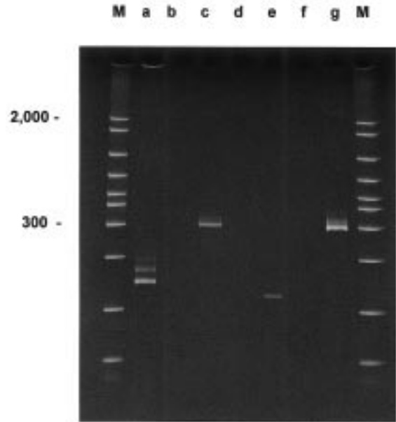
Fig. 5 Destruction of genomic RNA in viral particles by ESW-L The HIV-1 suspension was mixed with ESW-L, and amplified for LTR (lane b), pol (lane d) and gag (lane f) genes. The mixture with unelectrolyzed sodium chloride solution was examined in the same manner for LTR (lane a), pol (lane c) and gag (lane e) genes. The positive-control pAW109 RNA was well amplified in the assay (lane g). Lane M indicated marker for bp.
