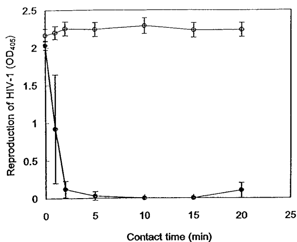
Fig. 1 Inactivation of infectivity of dried-HIV-1-infected cells
