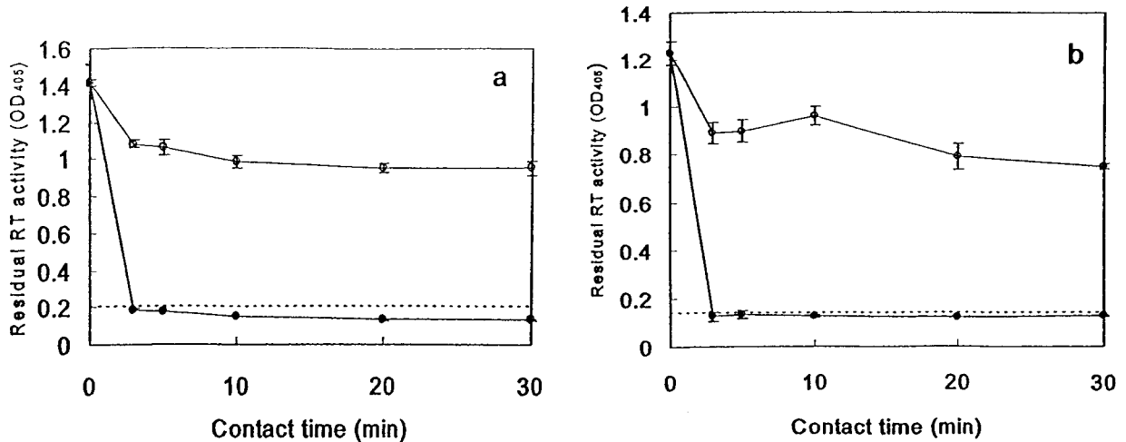
Fig. 3 Inactivation of enzymatic activity of HIV-1 RT a: Recombinant HIV-1 RT solution was treated with ESW-L (closed circles) or unelectrolyzed sodium chloride solution (open circles), and measured for RT activity. b: Viral solution was treated with ESW-L at room temperature, and measured for RT activity (closed circles). The viral solution was mixed with unelectrolyzed sodium chloride solution, incubated at room temperature, and measured for RT activity (open circles). Dotted line represents the cutoff line for the detection of HIV-1 RT activity in the culture supernatant.
