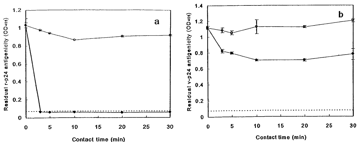
Fig. 2 Inactivation of antigenicity of HIV-1 structural protein p24 a: A solution of recombinant HIV-1 p24 protein was mixed with ESW-L, incubated, and measured for antigenicity (closed circles). A mixture of the solution and unelectrolyzed sodium chloride solution was incubated and measured for antigenicity (open circles). b: A mixture of viral suspension and ESW-L were incubated at room temperature and measured for the antigenicity of the recombinant HIV-1 p24 protein (closed circles). Unelectrolyzed sodium chloride solution was mixed with viral suspension, incubated for the designated time, and measured for antigenicity (open circles). Dotted line represents the cutoff line for the detection of the antigenicity of the HIV-1 structural protein p24.
